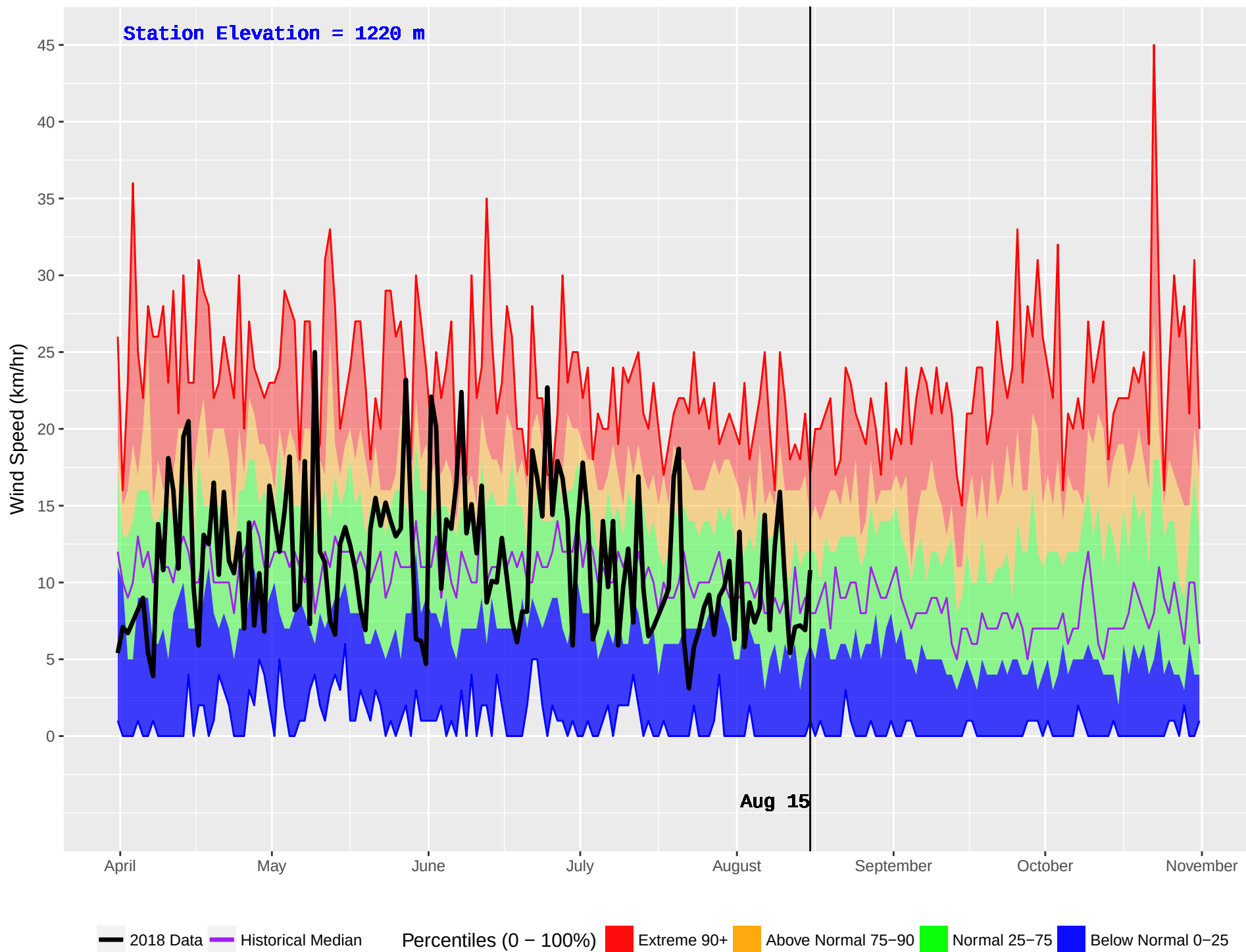
NEMIAH (216) : Historical (1982–2016) and Current (2018) Daily Wind Speed
