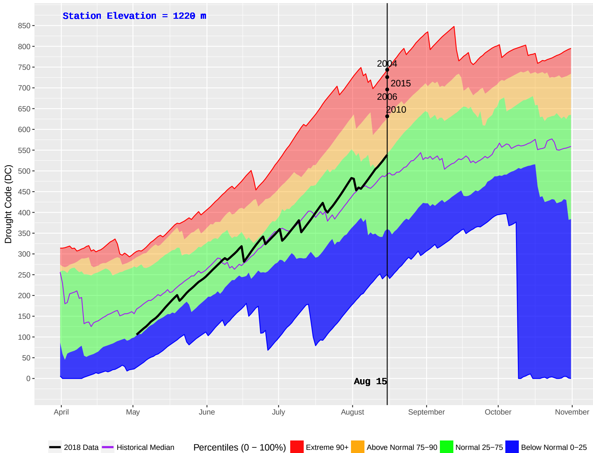
NEMIAH (216) : Historical (1982–2016) and Current (2018) Daily Drought Code (DC)
