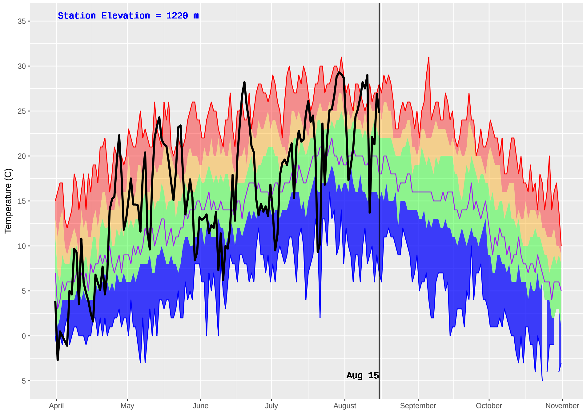
NEMIAH (216) : Historical (1982–2016) and Current (2018) Daily Temperature
